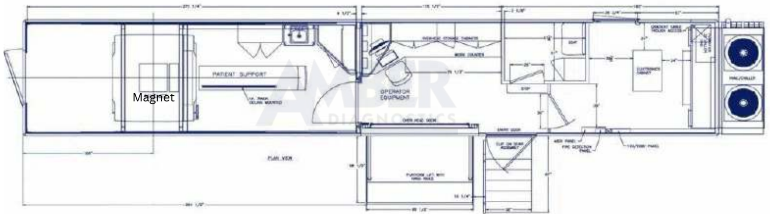
Mobile MRI Blue Print Top View
