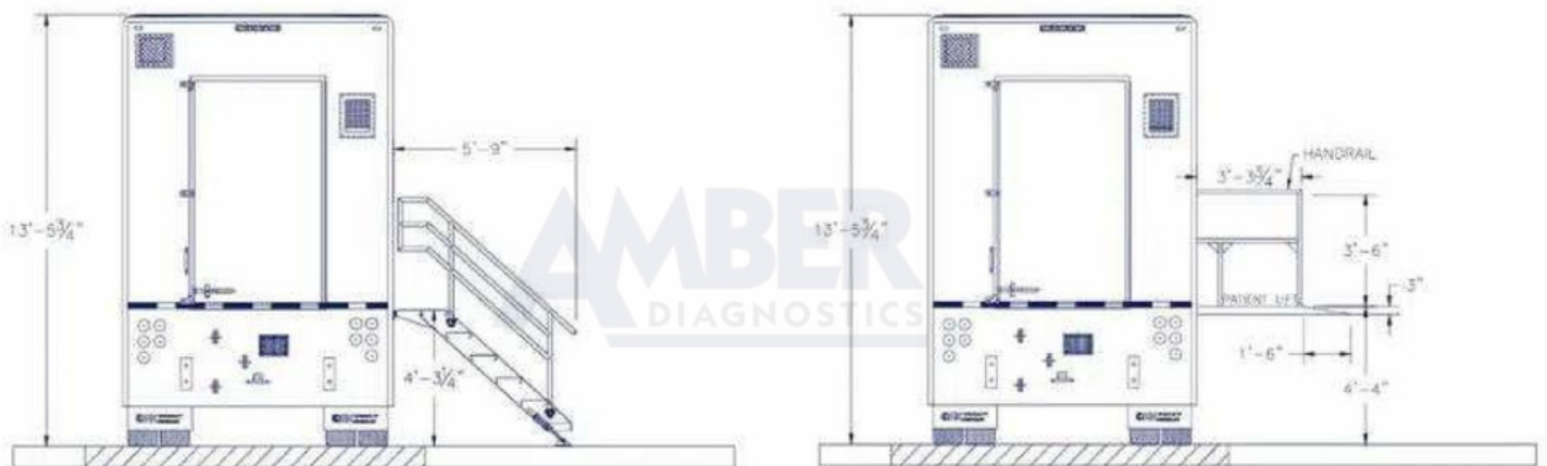
Mobile MRI Blue Print back view
